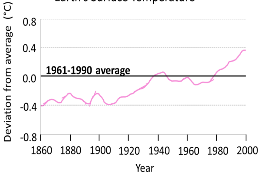
Earth's Surface Temperature
